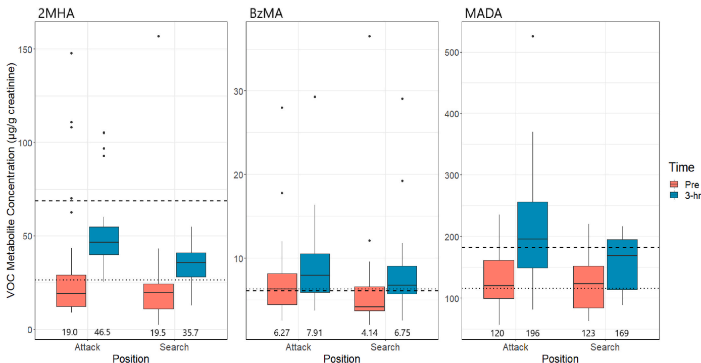
Fig. 1. Summary of urinary VOC metabolites ( \mu\text{g/g} creatinine) with medians included at the bottom of each plot for the residential fire study participants stratified by position for analytes that increase significantly post-fire. The number of firefighters in each position (attack and search) is 24. Dashed and dotted lines represent VOC medians of smoking and non-smoking general population, respectively.
